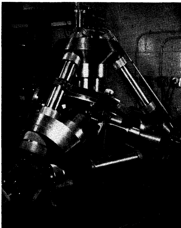
FIG. 2. Tetrahedral high pressure, high temperature x-ray diffraction apparatus.
