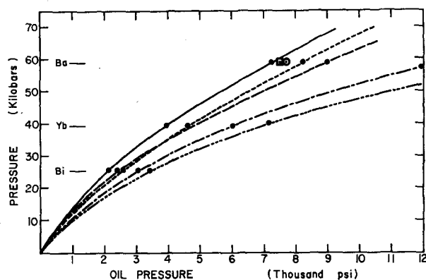
FIG. 5. Pressure calibration curves for the tetrahedral press using sample chambers of various x-ray transparent materials (anvils \frac{1}{4} in. on an edge, tetrahedron approximately 1 in. on an edge). Sample surrounded by polyethylene. — Pyrophyllite; - - - 50 wt% boron-filled plastic; - · - · 50-50 wt% boron-LiH; · · · · LiH coated with boron; - - - - LiH; □ 75-25 wt% boron-LiH; ○ 40 wt% boron filled plastic.
