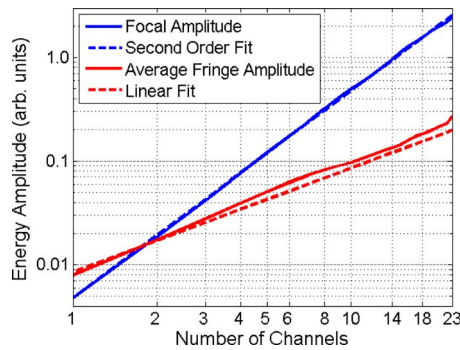
FIG. 3. (Color online) Focusing quality as a function of the number of channels used for TR. The focal energy and second order least-squares fit are displayed in blue (solid and dashed lines, respectively). The average fringe energy and first order least-squares fit are displayed in red (solid and dashed lines respectively).
