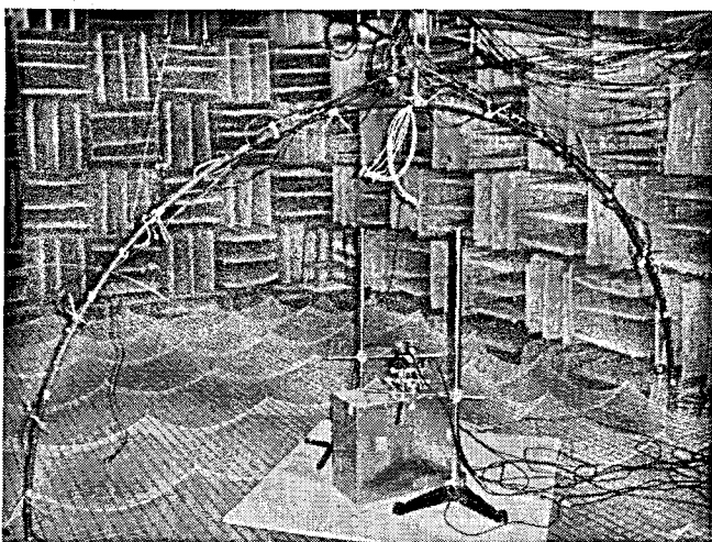
Fig. 6—An aluminum mock computer casing shown under a rotating semicircular microphone boom located in the anechoic chamber on the Brigham Young University campus.
