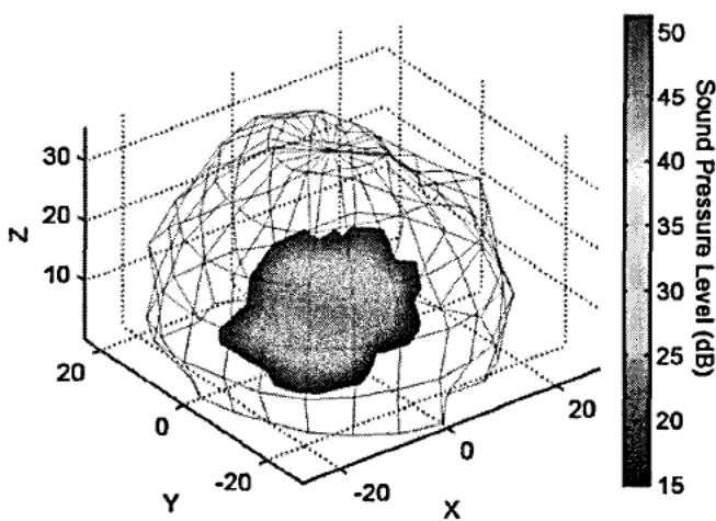
Fig. 10—Experimentally measured far-field acoustic pressure at 1110 Hz ( 3 \times BPF) for the 80-mm fan, without and with control. The wire mesh indicates control off, with radius indicating sound pressure level in that direction. The shaded surface indicates control on, with radius and color scale indicating sound pressure level.
