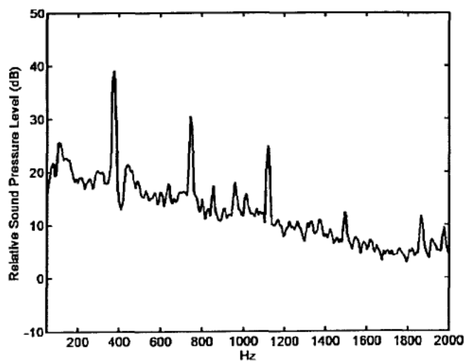
Fig. 1—A typical power spectrum of fan noise consisting of both broadband and tonal noise.
