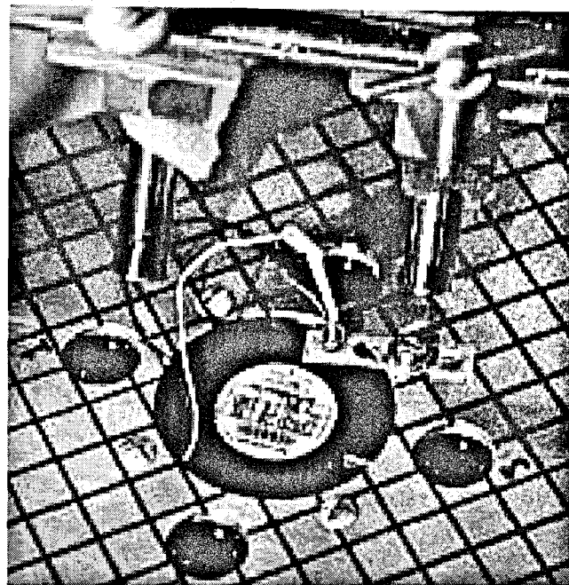
Fig. 7—The 60-mm fan surrounded by four 20-mm miniature loudspeakers.
