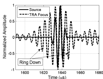
FIGURE 6: Comparison of the original input waveform (solid line) and the time reversed focus waveform (dashed line). Both waveforms are normalized to their respective peak envelope amplitudes. Note the broadening in time of the reconstructed source in the time reversed focal signal relative to the source pulse.
