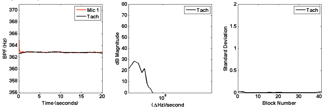
Figure 5: Low pressure and low speed case: Fan #3, 0 Pa pressure drop, 60% duty cycle PWM signal BPF vs. time (left), FFT of BPF vs. time (middle), Standard deviation of BPF vs. time (right)
