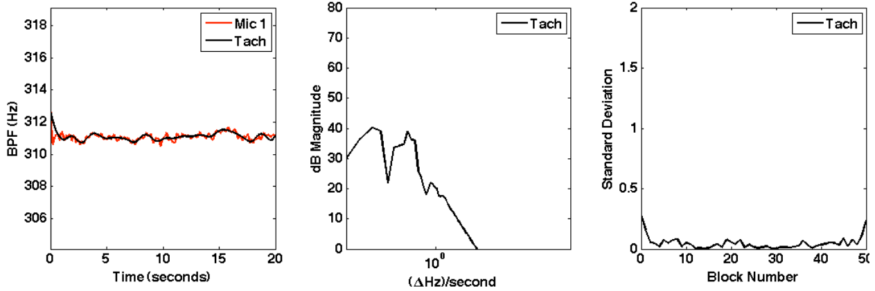
Figure 1: Low speed case: Fan #1, 24.9 Pa pressure drop, 60% duty cycle PWM signal BPF vs. time (left), FFT of BPF vs. time (middle), Standard deviation of BPF vs. time (right)
