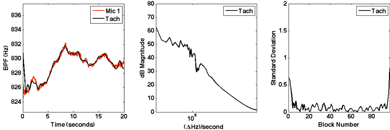
Figure 4: High pressure case: Fan #2, 24.9 Pa pressure drop, 15V constant driving voltage BPF vs. time (left), FFT of BPF vs. time (middle), Standard deviation of BPF vs. time (right)
