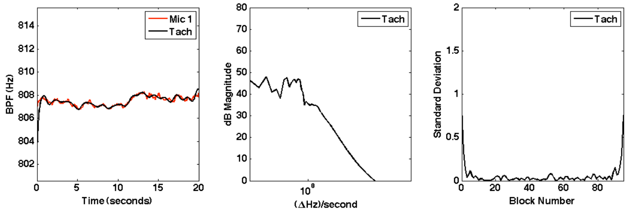
Figure 3: Low pressure case: Fan #2, 0 Pa pressure drop, 15V constant driving voltage BPF vs. time (left), FFT of BPF vs. time (middle), Standard deviation of BPF vs. time (right)
