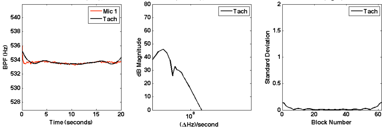
Figure 6: High pressure and high speed case: Fan #3, 24.9 Pa pressure drop, 80% duty cycle PWM signal BPF vs. time (left), FFT of BPF vs. time (middle), Standard deviation of BPF vs. time (right)
