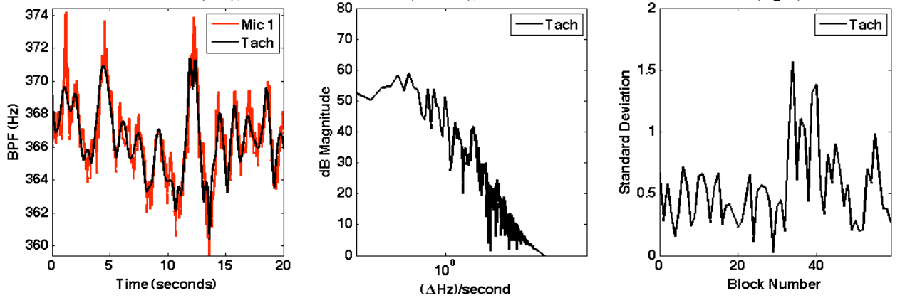
Figure 2: High speed case: Fan #1, 24.9 Pa pressure drop, 80% duty cycle PWM signal BPF vs. time (left), FFT of BPF vs. time (middle), Standard deviation of BPF vs. time (right)
