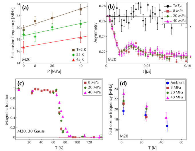
FIG. 4. (a) Increase of the oscillation frequency in the fast-relaxing portion of the muon decay asymmetry, for T = 2 K (superconducting), 25 K, and 45 K for \text{BaFe}_{1.9}\text{Co}_{0.1}\text{As}_2 [11]. (b) Muon decay asymmetry at 25 K as a function of uniaxial pressure. The fraction of muons remaining polarized in this short-time window are those landing in the nonmagnetic sample holder. (c) Fast-relaxing fraction of muons in a 30 G transverse magnetic field, demonstrating a constant magnetic sample volume below T_N = 65 K, as well as a broadening of the magnetic transition under pressure and an increase in T_N . (d) Data in (a) plotted as an order parameter.
