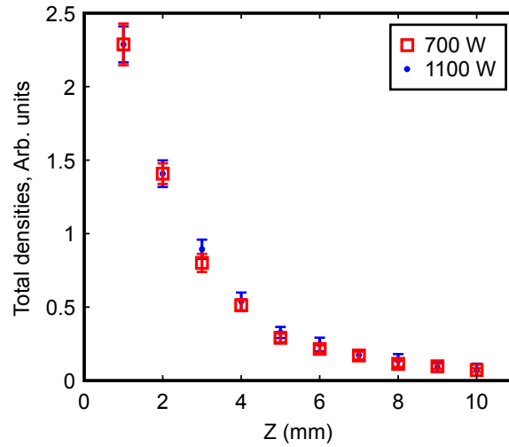
Figure 5.5 The result of least squares fitting to the total calcium density (Eq. 5.5). The error bars were calculated using Gaussian error propagation on the experimental data. These densities have not been scaled by the factor G(z) .
