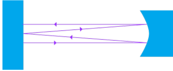
Figure C.1 Illustration of the optical path that makes a complete trip around the semiconfocal cavity. Note that the ray traverses the entire length of the path four times before doubling back on itself. It traverses the path 8 times before ending up in the same place again. This diagram similar to one found on page 277 of Ref. [55]. Here, we assume that the ray travels nearly parallel to the central axis of the cavity so that the length of each leg is well-approximated by the length of the cavity, L .
