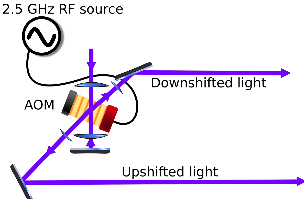
Figure 5.2 Detail of Figure 2.2. The light from the master laser is depicted entering from the top of the diagram. This beam travels into the AOM, which is depicted in the center of the diagram. The up-shifted light (up-shifted in frequency, or blue shifted) is depicted travelling towards the lens and mirror near the lower left side of the diagram. The zeroth order diffracted beam is re-collimated and then retroreflected. The down-shifted light (red shifted) is depicted exiting the AOM towards the top right of the figure.
