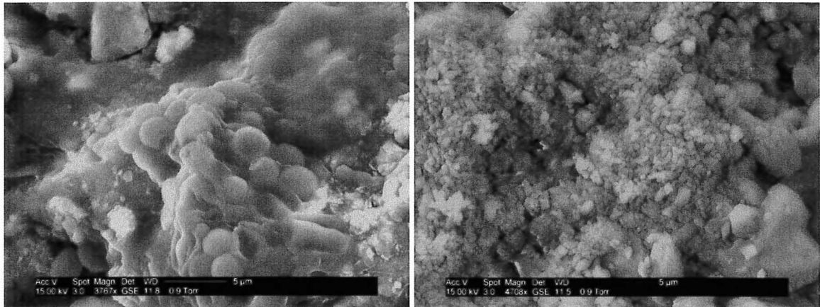
Figure 9 – On the left, an e-SEM photomicrograph of sample showing endolithic colony (2-3 micron spheroidal and associated amorphous structures) on a surface of a rock that fractured at the green endolith level. The organisms appear to be coated by a natural layer which obscures depth information. Angular material can be seen towards the lower corners of the photo. Under higher resolution these are seen to be crystals the chemical analysis of which shows much more Ca C and O than the endoliths or the underlying sand. Carbonates are known to bind sand stones together and may fulfill that role here. An image of a non-organic region of the rock is shown on the right, at the same scale.
