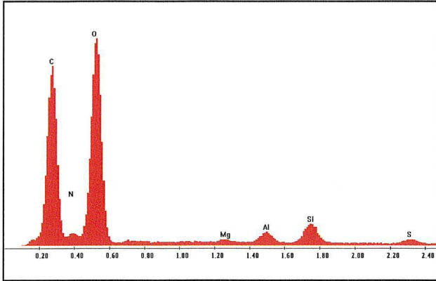
Figure 10 - Energy dispersive x-ray spectra of the elemental composition of a clump of endoliths in the E-SEM photo. Note that nitrogen is seen. N is not seen anywhere else on the samples in the CaCO 3 crystals and other clearly inorganic portions of the samples and is thus taken as evidence that the structures we have identified as cells are definitely biological in origin
