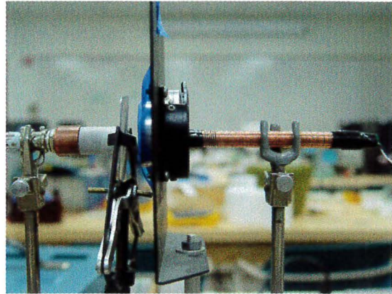
Figure 8 – A side view of our setup. From left to right: photodiode in a copper tube; steel aperture with 1mm diameter pinhole; aluminum mount holding the sample; LED mounted to a tube shielded with copper wire.
