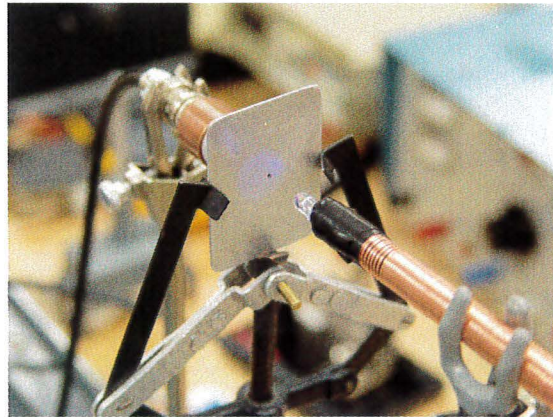
Figure 7 – A photograph of the experimental setup. The LED is shining onto the steel aperture.
