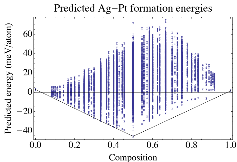
Figure 4.6: Predicted CSCE formation energies obtained using the ECI’s shown in Fig. 4.5; error bars are standard deviation due to different random choices of \leq 400 structure subsets. Black solid line denotes the convex hull calculated from the average energies; only Ag, Ca 7 Ge-type Ag 7 Pt (barely, with a depth of less than 1 meV/atom), L 11 AgPt, and Pt are predicted to be T = 0 K ground states.
