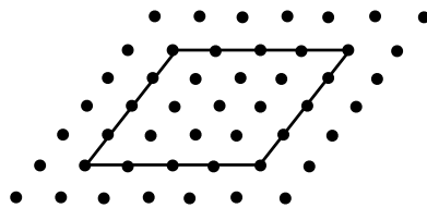
Figure 2.3: Illustration of the Monkhorst-Pack scheme for choosing k -points. Rectangular (left) and triangular (right) reciprocal unit cells are shown. For the rectangular unit cell, the k -points mesh is defined by dividing one lattice vector into 4 divisions and the other into 3, creating a mesh of uniform density. For the triangular unit cell, the mesh is defined by dividing both lattice vectors into 4 divisions. In each case the choice of division is dictated by the requirement that the density of the mesh be uniform.
