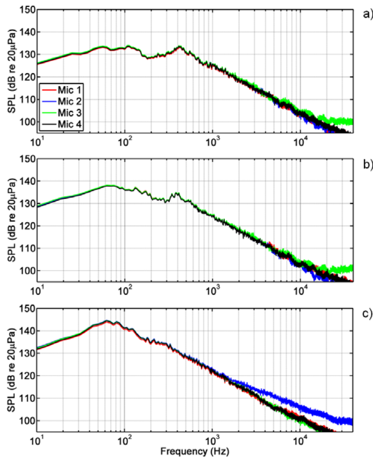
Figure 6.10. Sound pressure level for the a) EF3, b) EF2, and c) SA1 arrays during the GEM60 test firing n June 2008. The individual plots are for arrays a) 11.1, b) 16.7, and c) 27.8D downstream.
