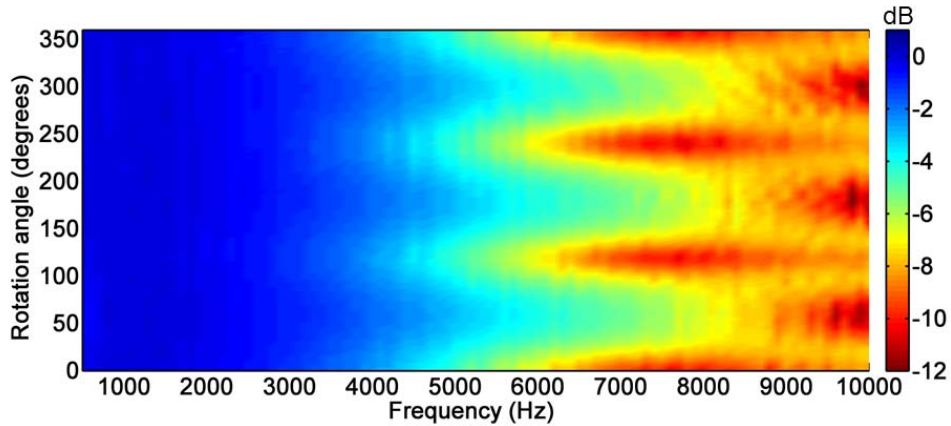
Figure 3.7. Intensity magnitude error relative to plane wave intensity calculated via Equation 3.1, utilizing the average squared pressure of the four microphones in the array for p_{\text{avg}}^2 .
