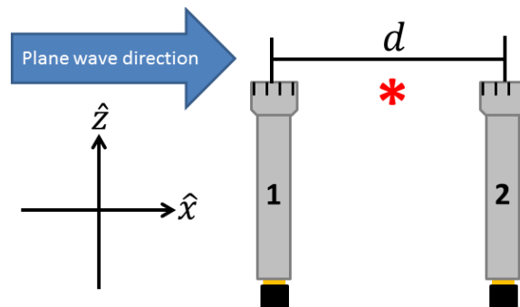
Figure A.1. One possible configuration for the p-p method for measuring acoustic intensity. Often times, the microphones are rotated to face each other and are separated by a spacer. The mathematical derivation of either orientation is the same.
