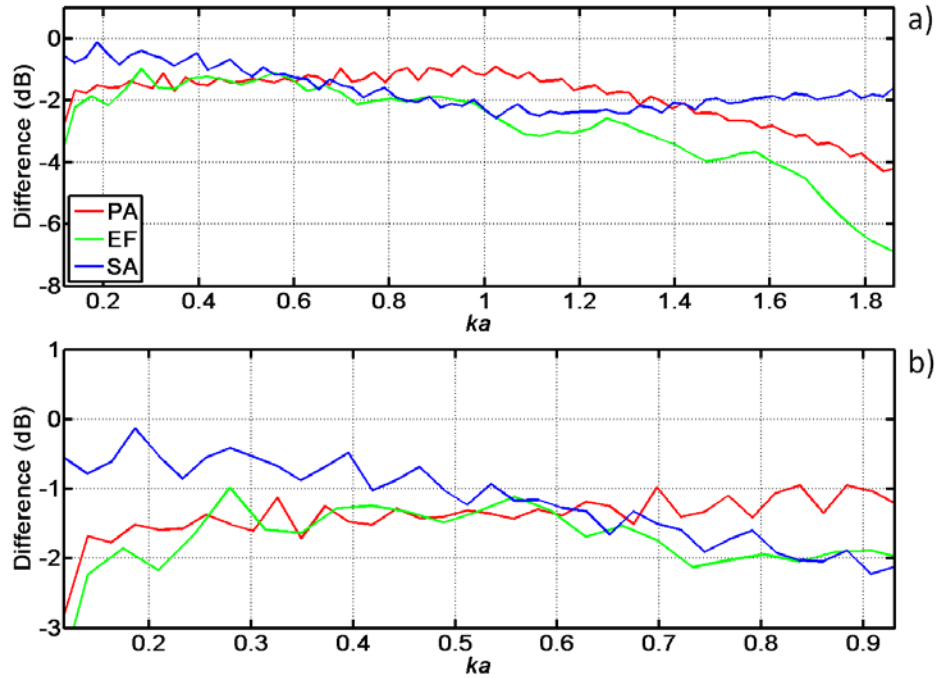
Figure 4.6. Difference between the potential and kinetic energy density levels for the PA, EF and SA arrays for a) 500 Hz to 8 kHz and b) 500 Hz to 4 kHz assuming a=1.27 cm.
