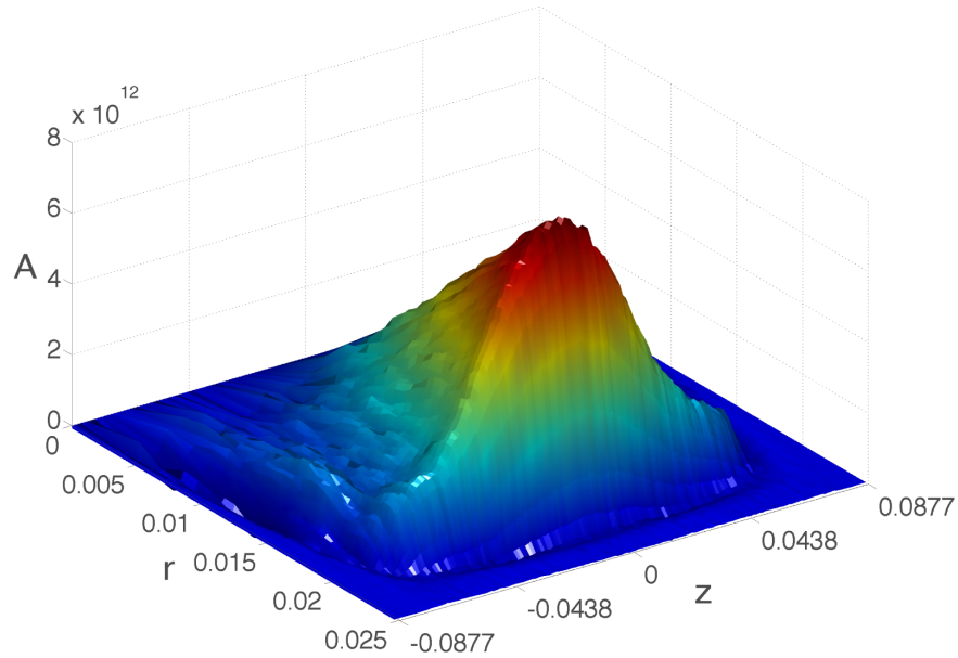
Figure 4.4. Mode shape for the main frequency peak with k_z = 1/2 (marked “C” in Figure 4.3).
