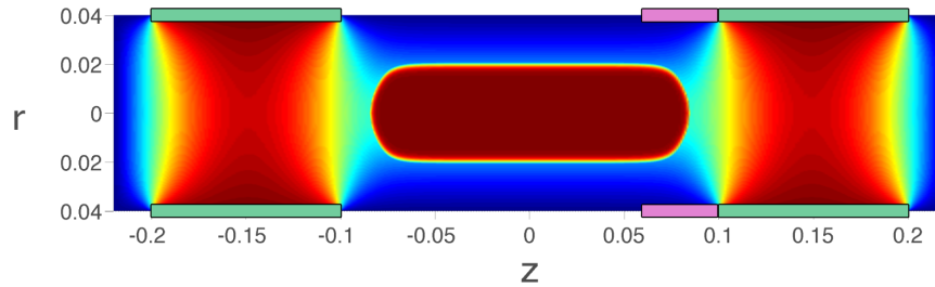
Figure 4.1. Overlaid colormap of the plasma density and confining potential inside the computation region. The green and purple rectangles represent the confinement (10 cm wide) and diagnostic (4 cm wide) rings respectively.
