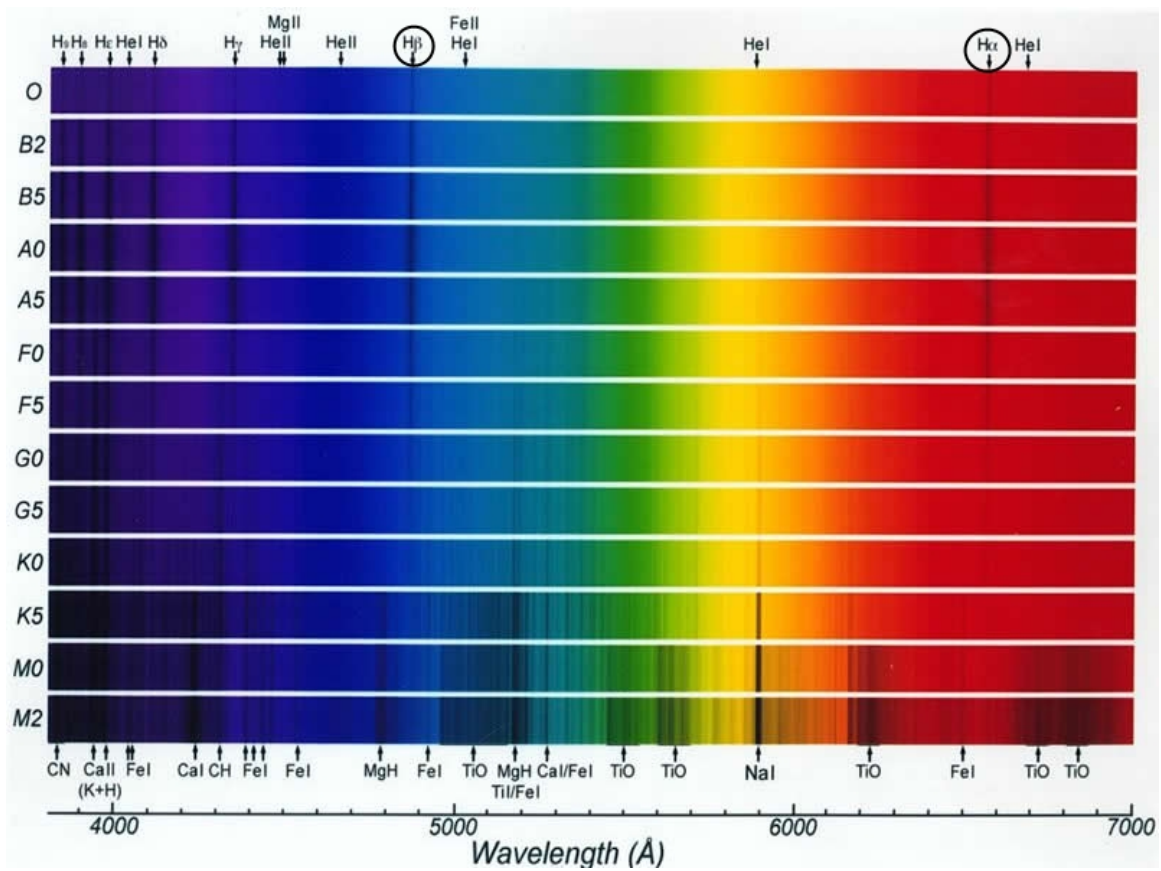
Figure 1.1 Spectra for stars of various spectral types. Image courtesy of academics.smcvt.edu
