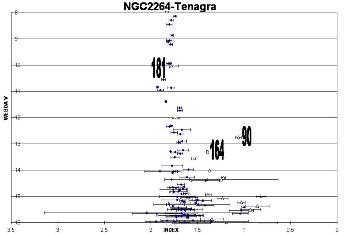
Figure 8: NGC 2264 Tenagra data. The horizontal axis is the H \alpha index defined as N-W. The vertical axis is the V values obtained for the stars from the WEBDA database. Open triangles were identified as emission objects by Sung et al. (1997) and emission candidates are shown by an x. Spectra were obtained for the three numbered stars (181-open circle, 90, and 164).
