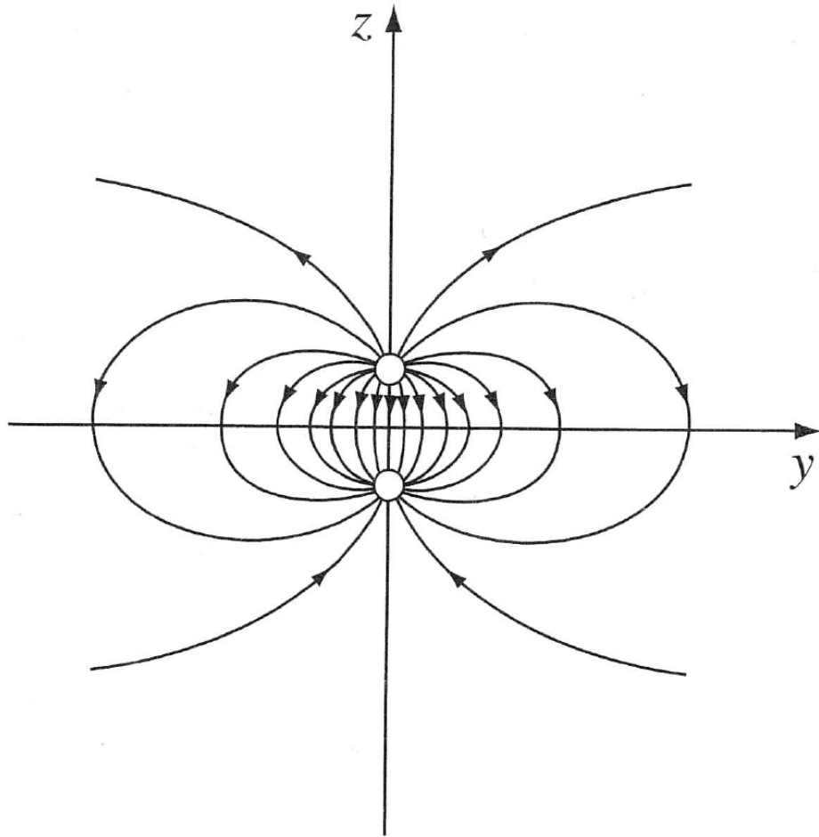
(b) Field of a "physical" dipole
