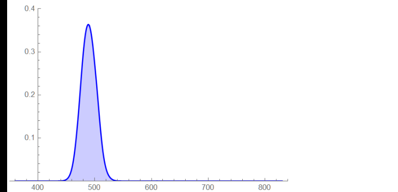
Projection of the intensity function onto the Z color matching function
