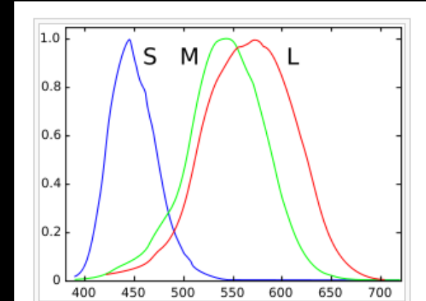
Cone cell response, again
