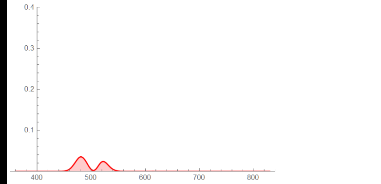
Projection of the intensity function onto the Y color matching function
