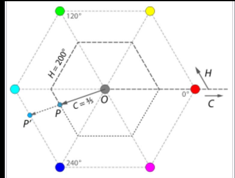
Fig. 9. Both hue and chroma are defined based on the projection of the RGB cube onto a hexagon in the "chromaticity plane". Chroma is the relative size of the hexagon passing through a point, and hue is how far around that hexagon's edge the point lies.
