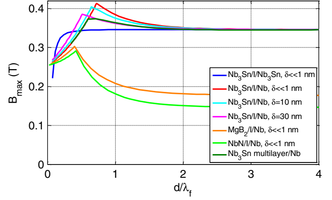
FIG. 2. Maximum field below B_{\text{sh}} of both the film and the bulk as a function of film thickness for various film materials in a SIS structure with Nb. The effect of varying the insulator thickness \delta is shown for the \text{Nb}_3\text{Sn} film, as is the effect of splitting the film thickness d over five equally thick multilayers with thin separating insulators. All calculations are done in the London limit.
